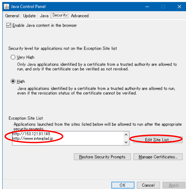
Java Control Panel [Security] window
