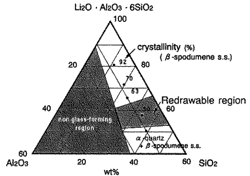
Fig. 2 Redrawable region of \text{Li}_2\text{O}-\text{Al}_2\text{O}_3-\text{SiO}_2 glass-ceramic.
