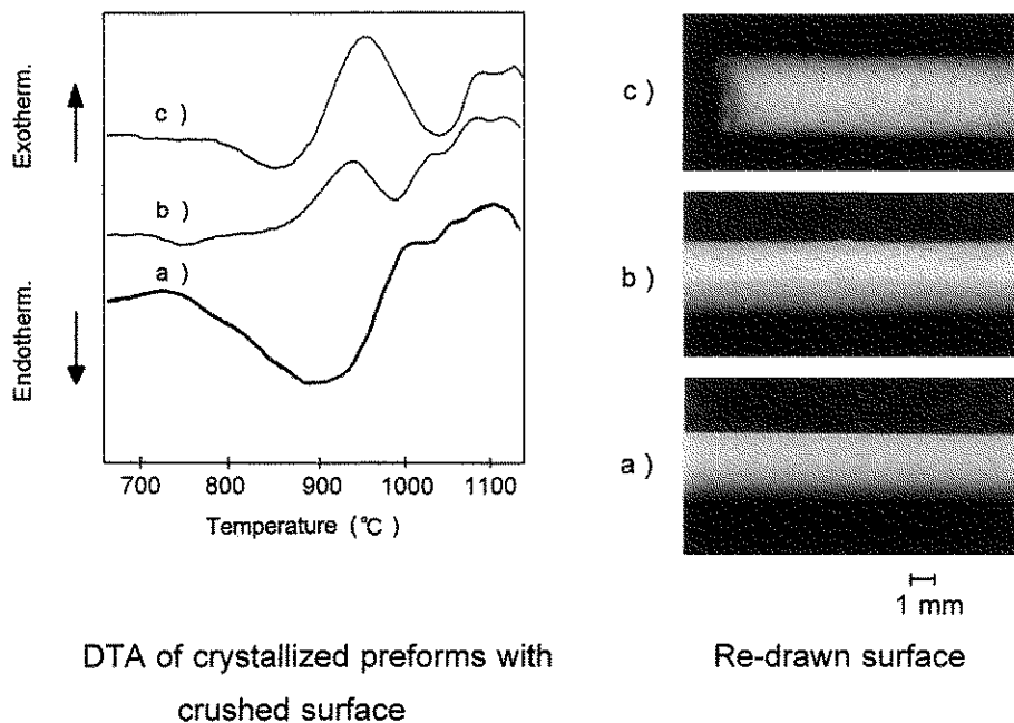
Fig. 4 DTA behavior of cerammed preforms and surface devitrification of redrawn capillaries.
