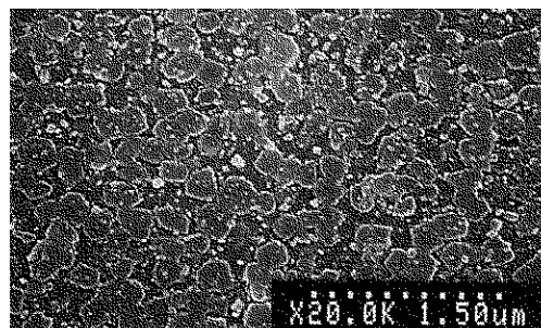
Fig. 5 Crystalline structure of the cerammed preform.
