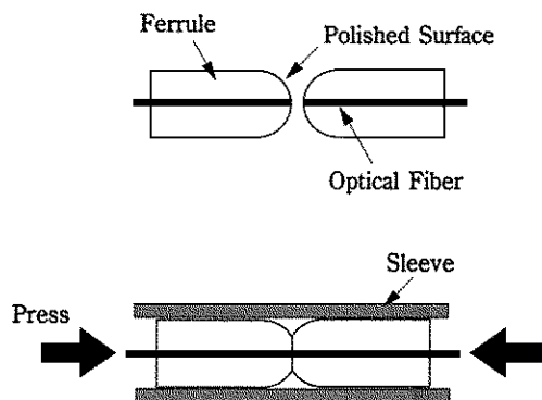
Fig. 1 Connection mechanism of optical fibers.
