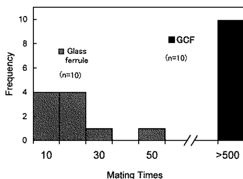
Fig. 8 Scratch resistance of GCF.
